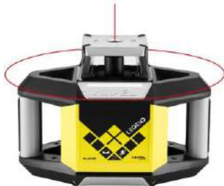
NL300R DIGITAL NIVEL SYSTEM
